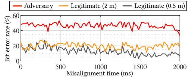
Fig. 7: Bit error rates under replay attack. Legitimate devices successfully authenticate using current ambient audio, while an adversary with replay attack fails to authenticate.
