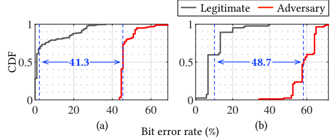
Fig. 8: CDF of bit error rates on (a) conversation audio and (b) cleaning audio
