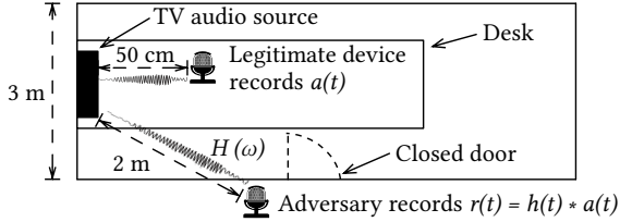
Fig. 5: A floorplan of testbed used to evaluate TREVOR.
